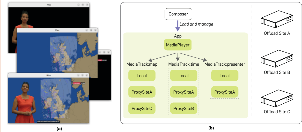
Figure 4. An example of a simple weather forecast (a), and a simplified software architecture for media playback (b).
